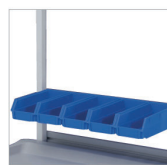
SBS-1 Bacs stockage vrac (L) 75 × 105 × 190 mm
